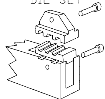
IDEAL/STANDARD DIE SET
